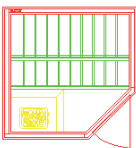
SKNL-1111 110x110x200cm 1 Person 3KW
